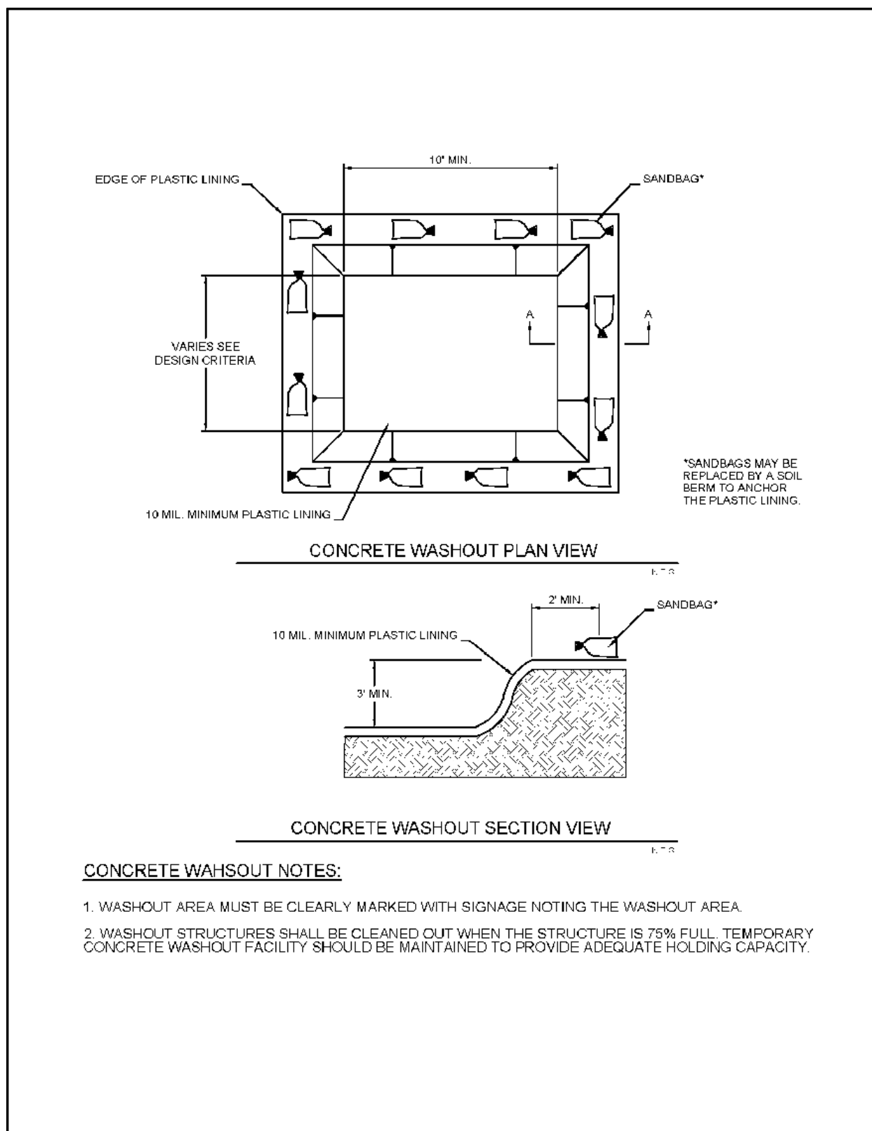
Figure 29: Schematic diagram of below-grade concrete washout installation
